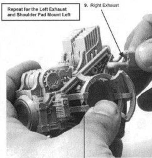
1. Shoulder Pad Mount Right
